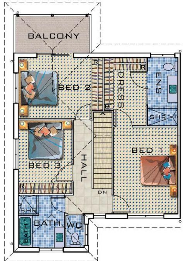
FIRST FLOOR SCALE 1:100
