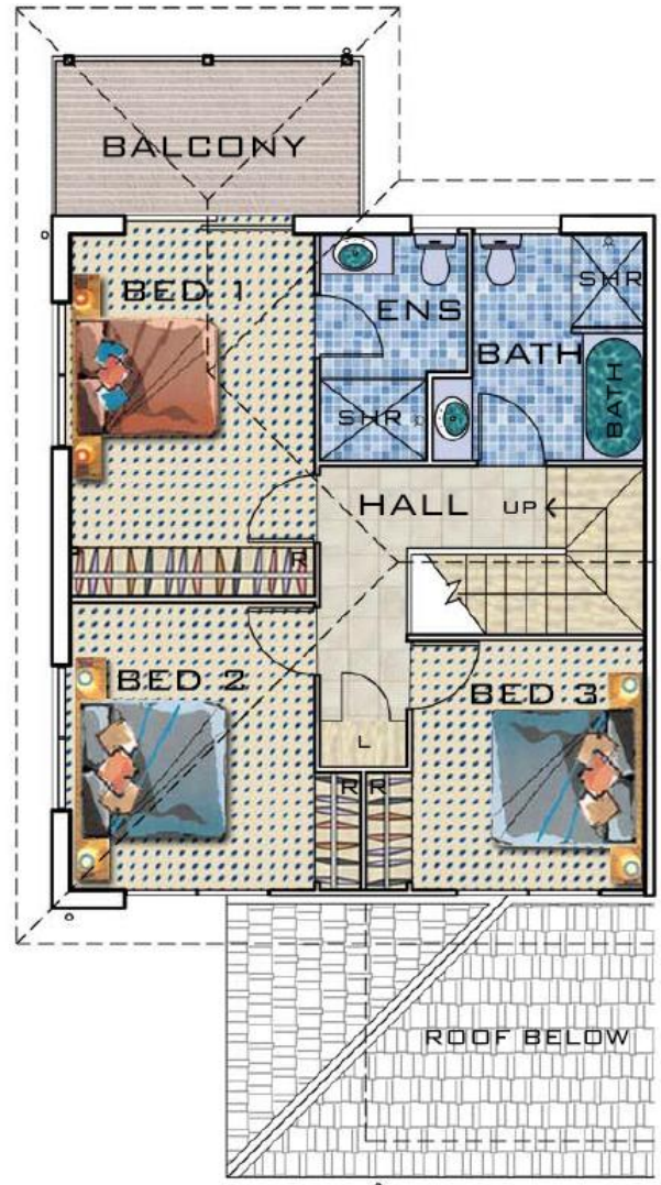
FIRST FLOOR SCALE 1:100
