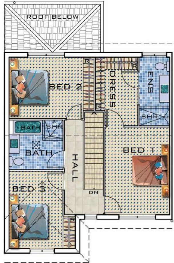
FIRST FLOOR SCALE 1:100
